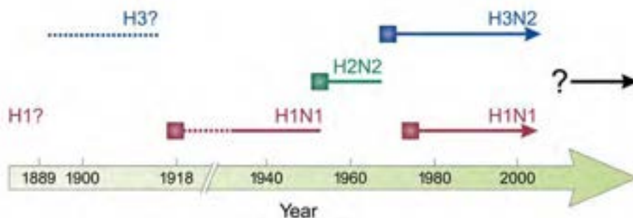
Influenza subtypes 266
